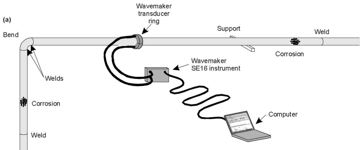
Figure (a), typical GWT equipment setup
