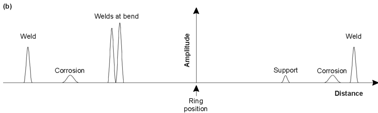
Figure (b), typical data obtained from GWT testing – relates to setup shown in Figure (a)
